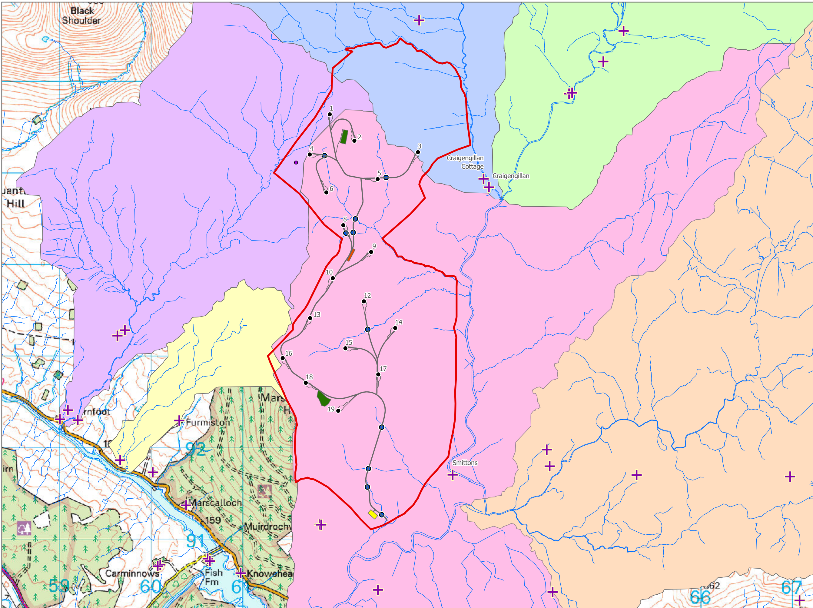
Figure 13.1: Hydrological Catchments
